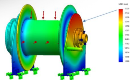
Displacement Analysis in Simulation
